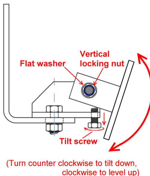
Fig 6.3-5 Vertical tilt
