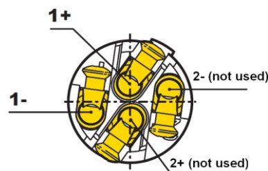
Fig 7.2-3 NL4FC pin-out
