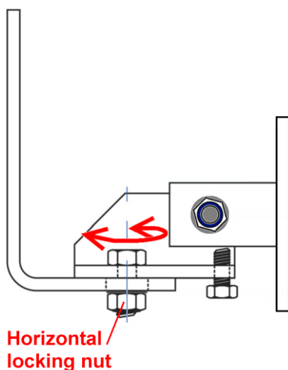
Fig 6.3-4 Horizontal swivel
